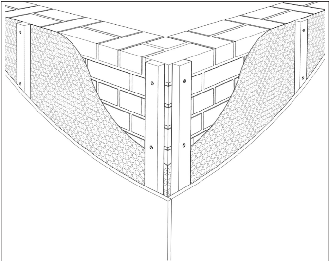
Figure 3 Typical external corner detail
