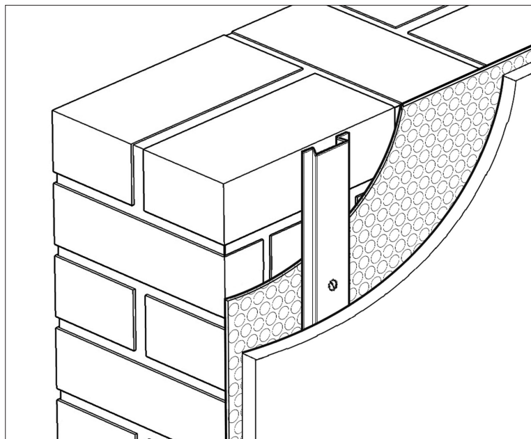
Figure 6 Metal furrings method
